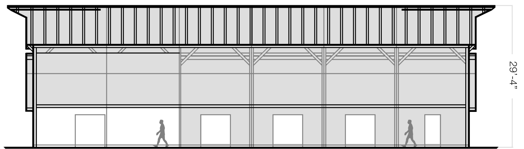
Side View
