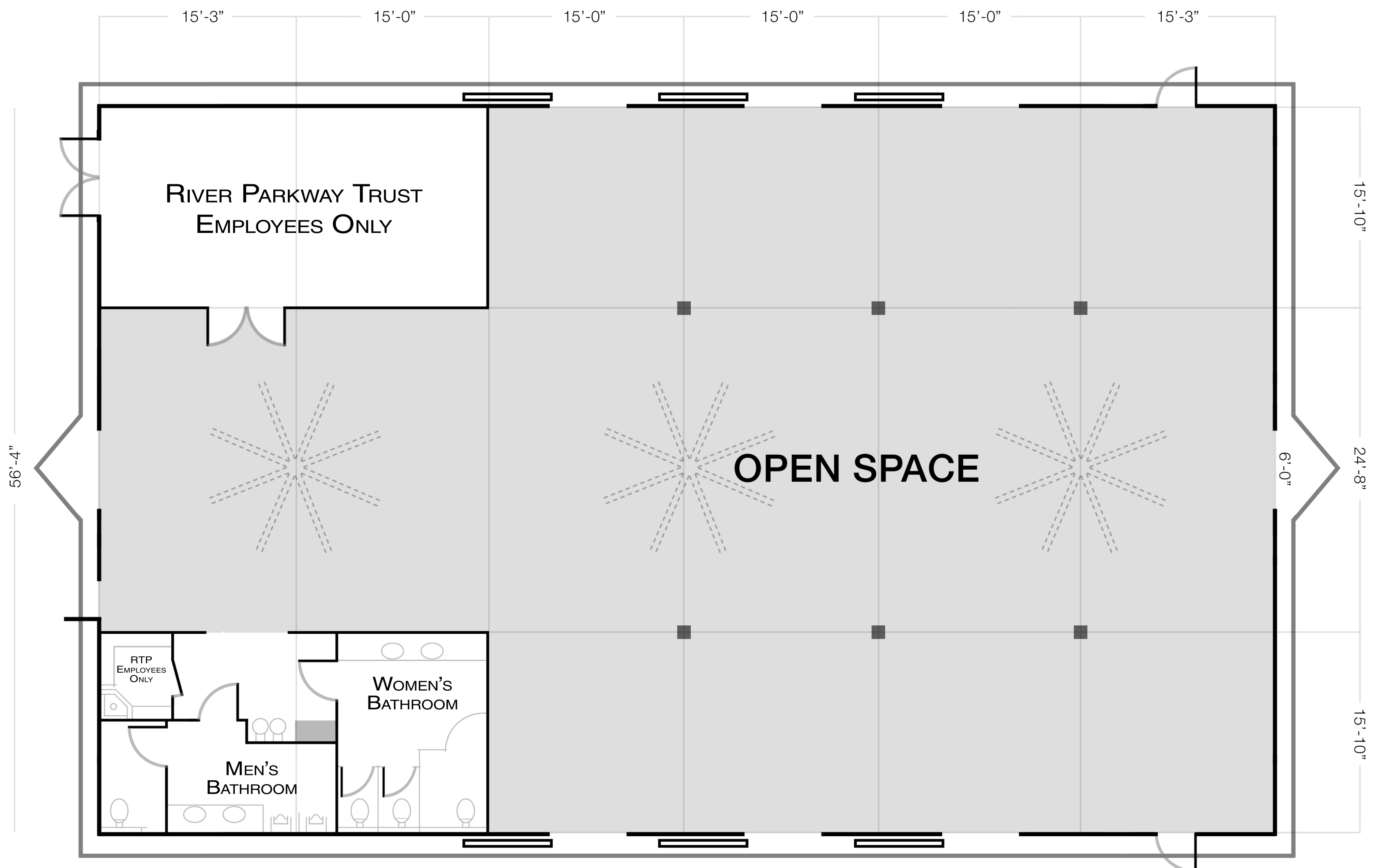
Floor Plan
