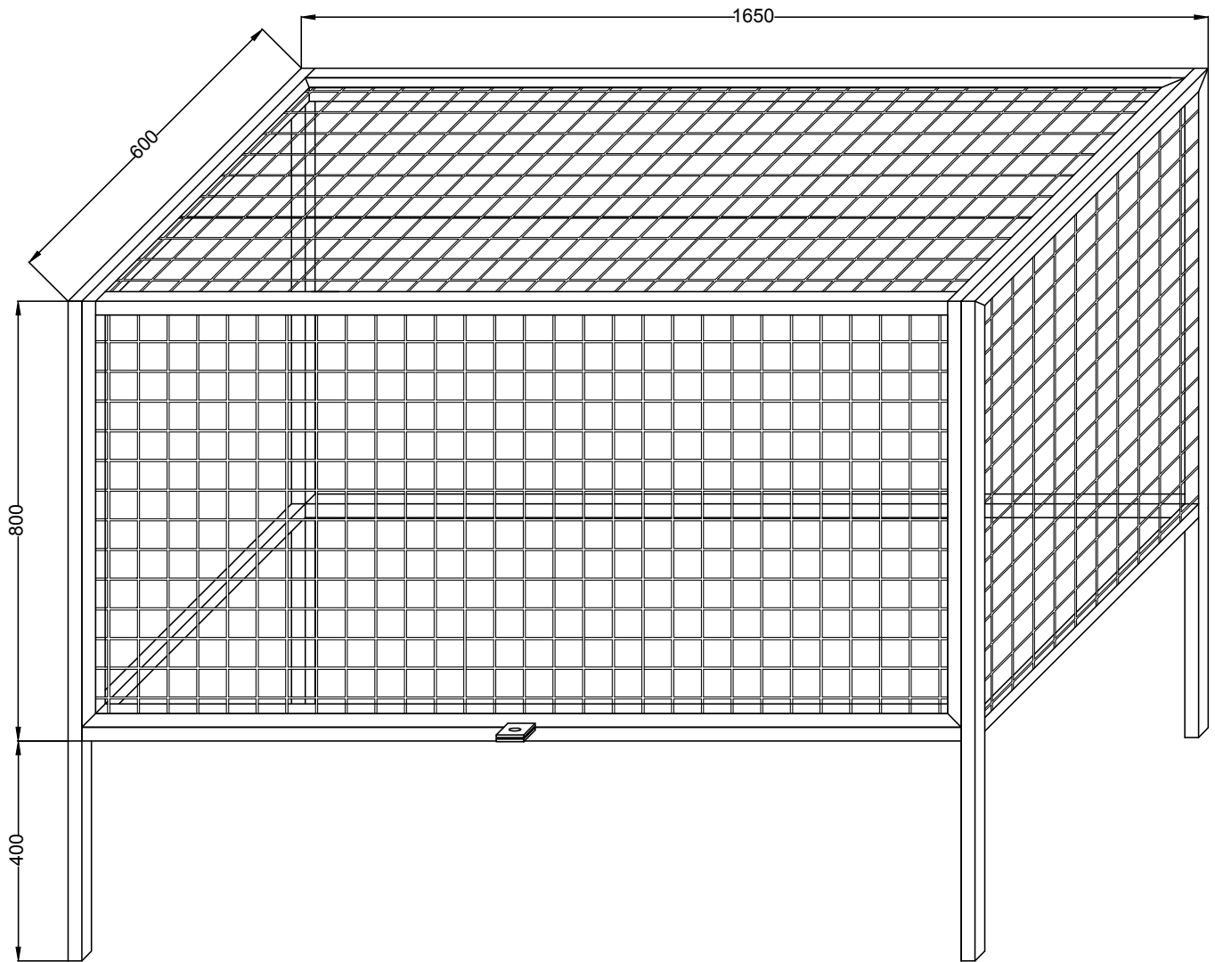
RPZD ENCLOSURE DETAIL
