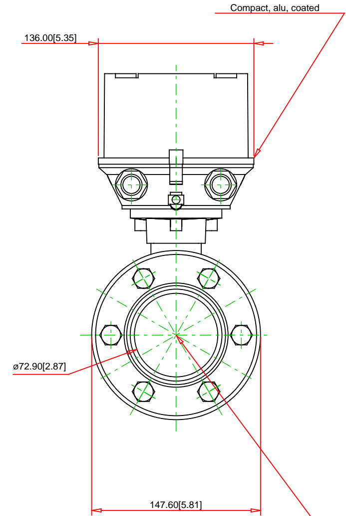
Tri-Clamp, ASME BPE, 1.4404/316L, for pipe size: DN2-8=1/2", DN15=3/4", DN25=1"
