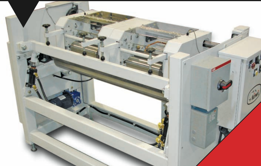
Model 2411THS. High speed printing capability, with narrow flexo laterally adjustable across wide web. Web speed matching, flexo base assembly and web pressure release also shown.
