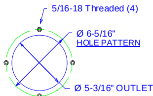
DUCT OPENING (OUTLET)
