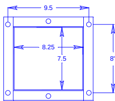
8.25x 7.5 Flat Flange (A)
