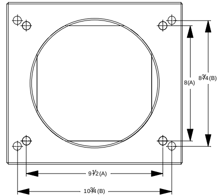
Mounting Hole Layouts
