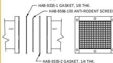
HAB-9586 Anti-Rodent Screen Supplied w/ 1/8\"/>
