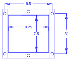
Mounting hole layout
