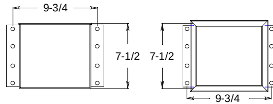
Mounting Hole Layout for all ducts on this page (male/female flange end per each duct)
