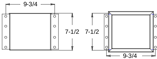
Mounting hole layout
